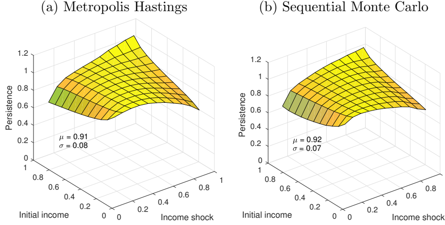
Figure 3: Comparing Metropolis Hastings and Sequential Monte Carlo in the balanced panel used in Arellano, Blundell and Bonhomme (2017, ABB)
