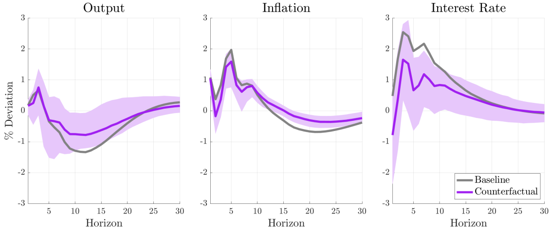
Figure 4: Output, inflation and interest rate impulse responses to a contractionary investment-specific technology shock under the prevailing baseline rule (grey) and the optimal policy rule for a dual-mandate policymaker ( \lambda_\pi = \lambda_y = 1 ) within the identified subspace (purple). The shaded areas correspond to 16th and 84th percentile confidence bands.
