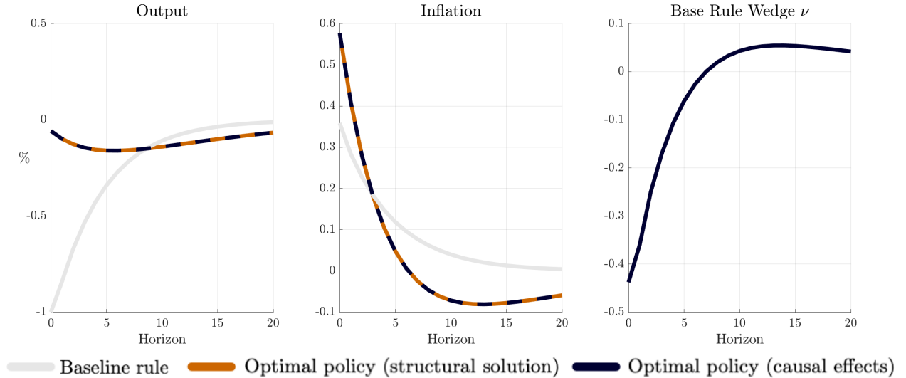
Figure 2: Output and inflation impulse responses together with the equivalence shock wedge \nu (see (22)) for the HANK model with policy rules (37) and the optimal policy given by (39). The impact output contraction under the prevailing baseline rule is normalized to -1\% .
