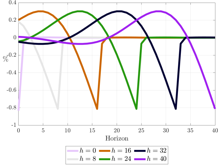
Figure A.1: Output impulse responses to contemporaneous and forward guidance monetary policy shocks in the HANK model of Appendix A.3.
