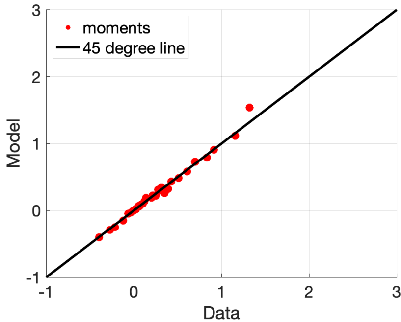
Figure C.1: Model Fit
