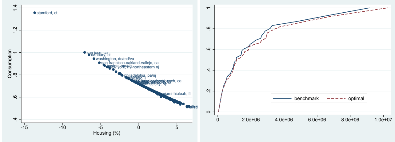
Figure 10: Implied changes of implementing the optimal policy \tau^* : A. Substitution between c and h ; B. Cumulative Distribution of city sizes.
