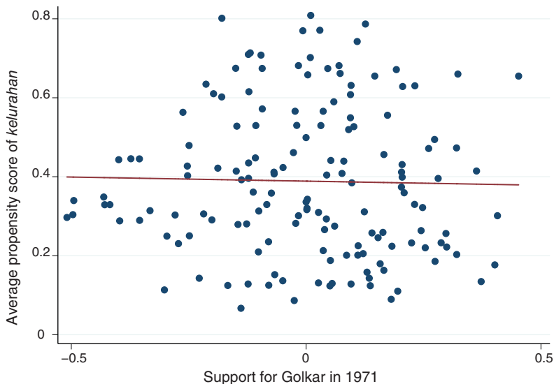
FIGURE 2. ENDOGENEITY CHECK
