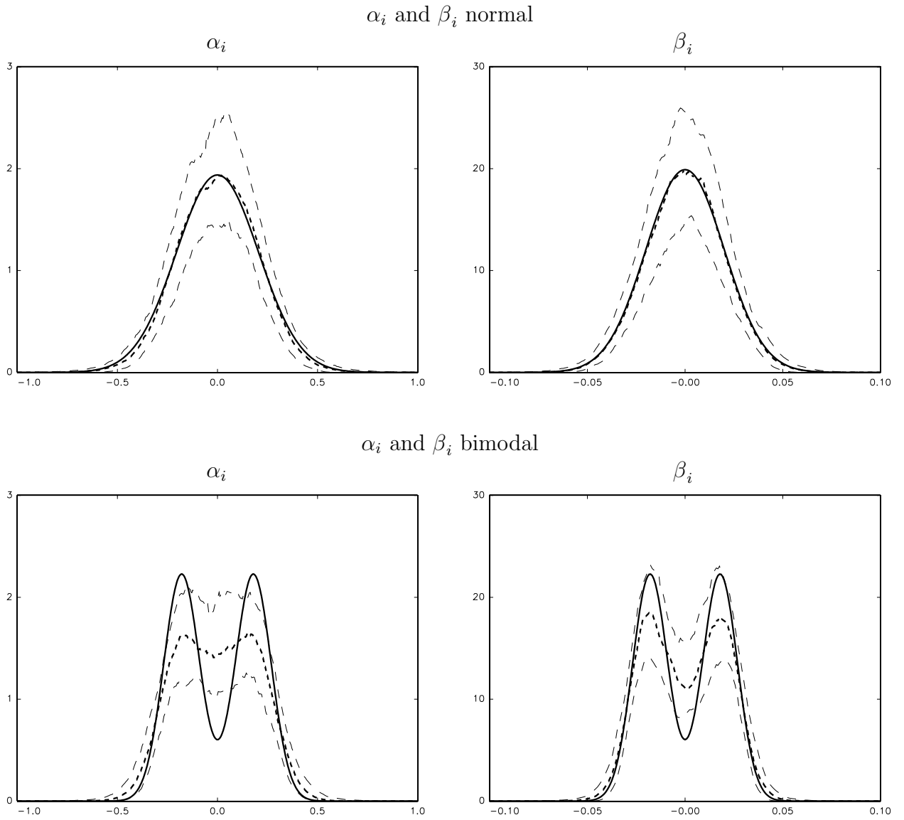
Figure F1: Density estimates on simulated data using Mallows' algorithm
